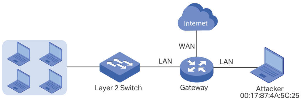
Figure 3-6 Network Topology
