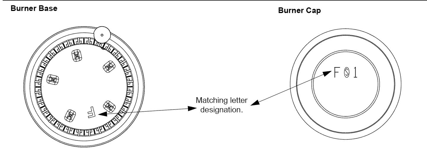
Figure 4: Burners Caps
