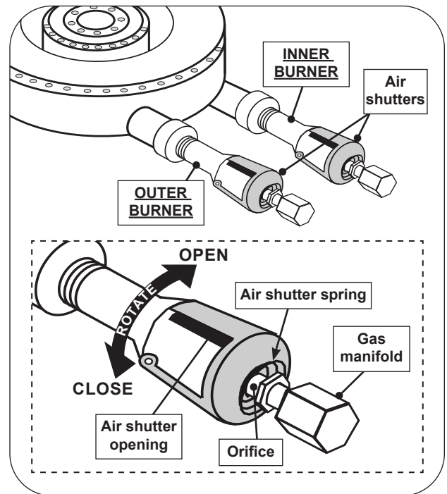
Fig. 42-1 Power burner air shutter adjustment detail
