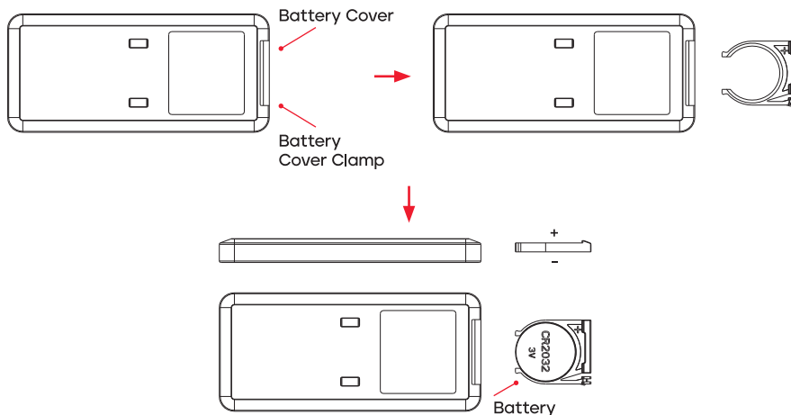
Remote Control
