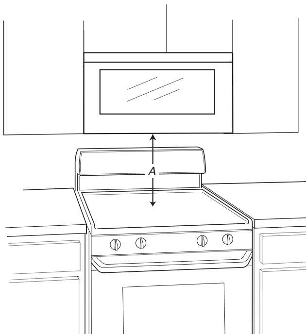
A. 12\frac{7}{8} " (33 cm) is the height from the highest point of the stove to the bottom of the microwave oven.
