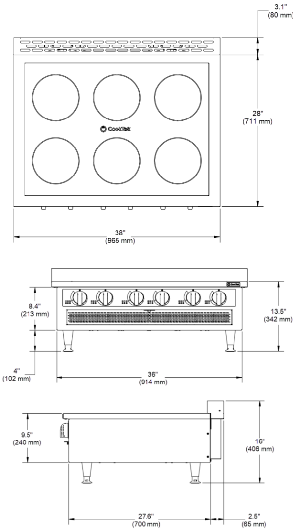
Figure 3-4: Six Hob Freestanding Dimensions
