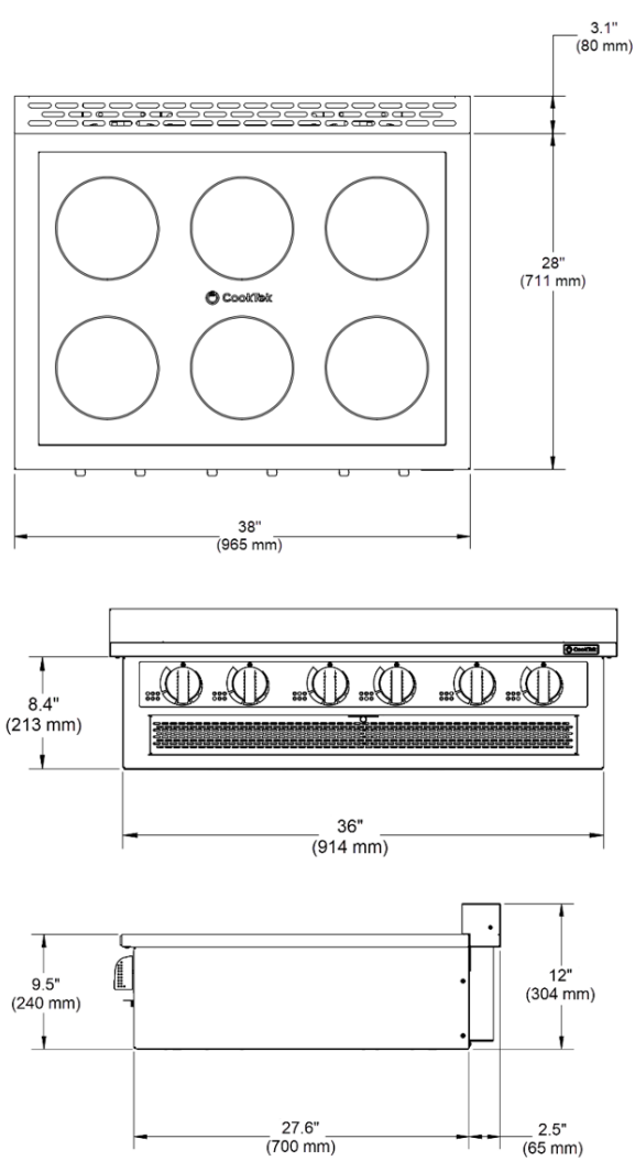
Figure 3-5: Six Hob Drop-In Dimensions
