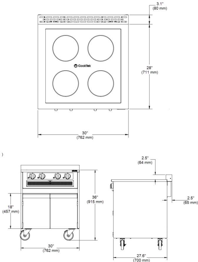
Figure 3-3: Four Hob Cart-Mounted
