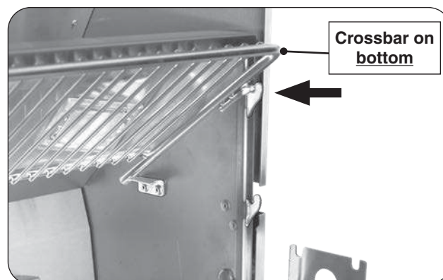
Fig. 24-4 Place warming rack in storage position
