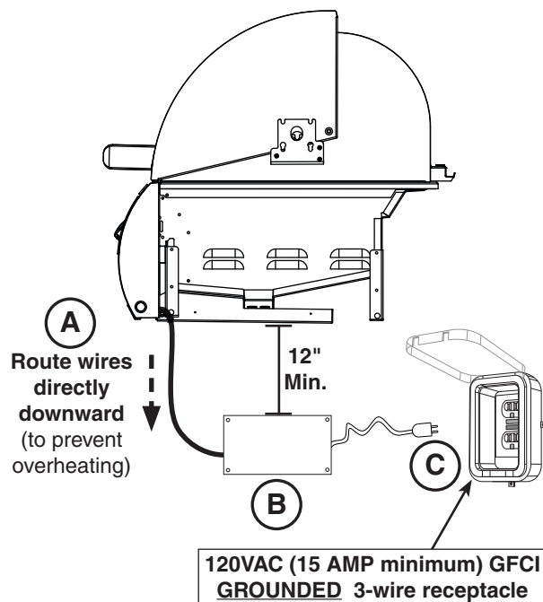
Fig. 25-1 Electrical installation
