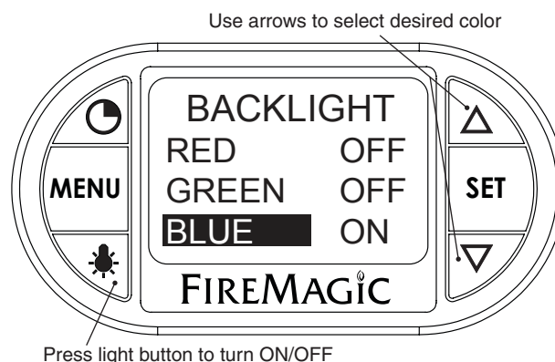
Fig. 32-2 Backlight screen
