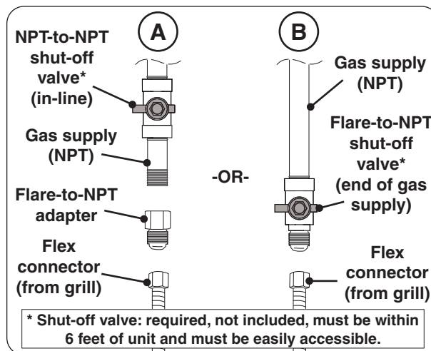
Fig. 22-1 Connecting to a gas line
