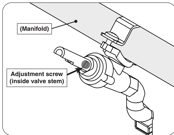
Fig. 46-3 Valve adjustment screw location
