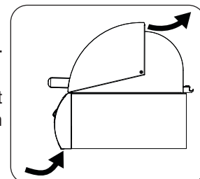
Fig. 27-1 Airflow diagram
