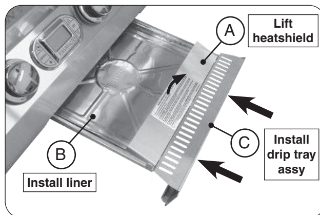
Fig. 24-1 Install drip tray
