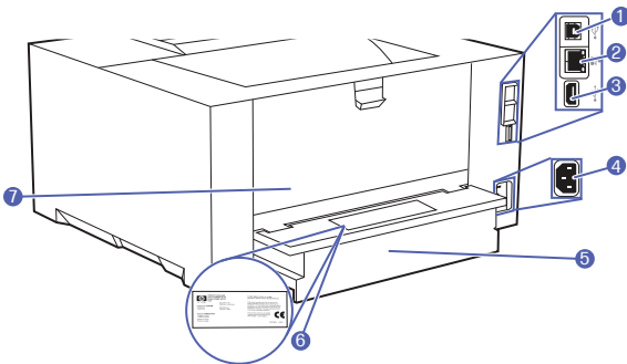
Figure 1-7 Printer rear view
