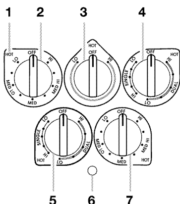
Knob Control
