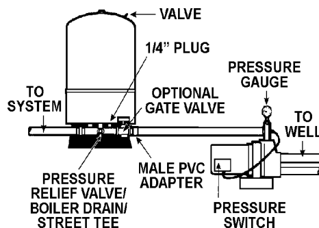
Figure 10. Base Mounted Jet Pump With Vertical Tank
