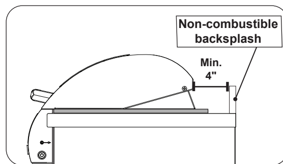
Fig. 17-2 Backsplash clearance
