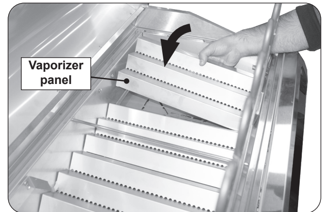
Fig. 29-2 Install vaporizer panels
