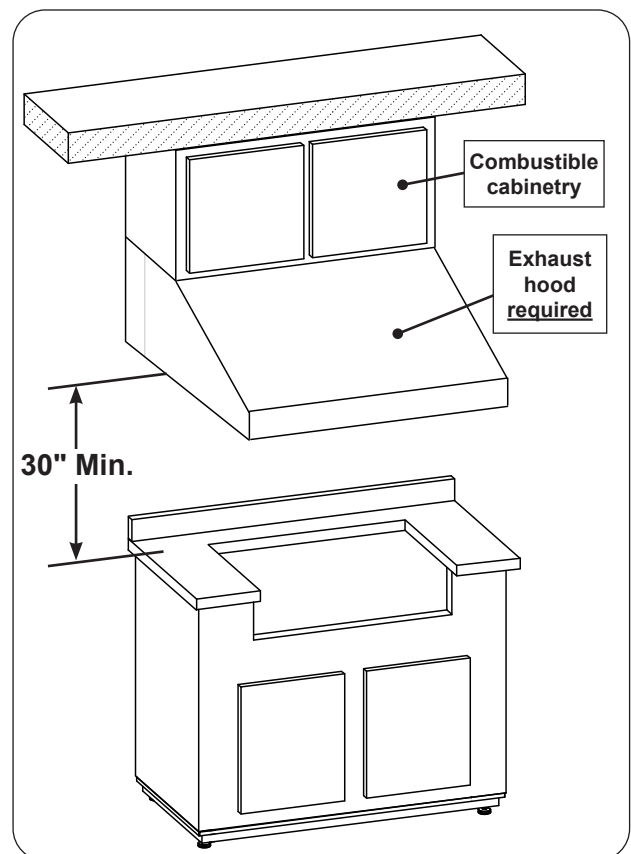
Fig. 16-2 Overhead cabinetry requirements
