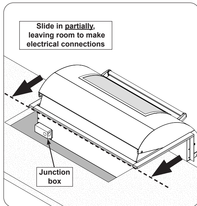
Fig. 27-2 Position unit for wiring
