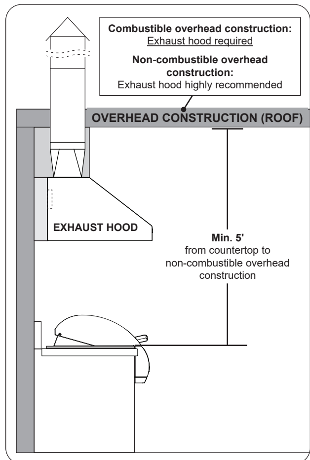
Fig. 16-1 Overhead (roof) requirements
