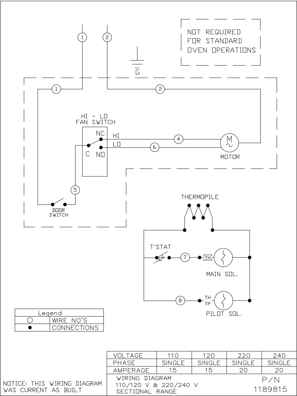
Figure 18 Wiring Diagram for Oven Base with Standing Pilot
