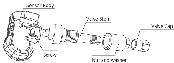
Metal Valve Sensor
