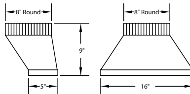
VP565 Standard Transition (Included)
