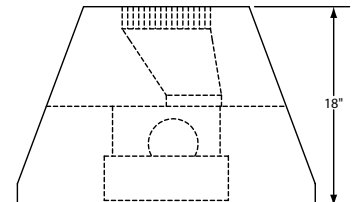
Transition Installed (Side View)
