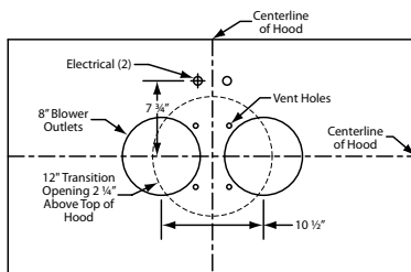
1100 CFM T400 Dual Blowers (Top View)
