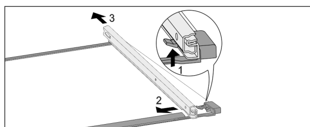
Fig. 59 Glass shelf with rails
