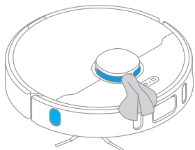
Clean the LDS Laser Sensor/Edge Sensor
