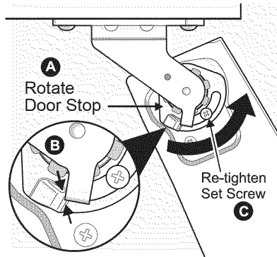
Retighten Screw
