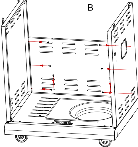
M4X10 screw Qty: 22 pcs
