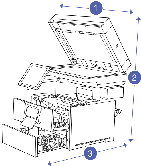
Figure 1-14 Dimensions for the printer opened
