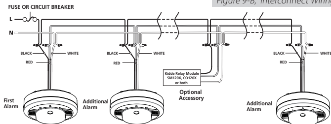
Figure 9-B, Interconnect Wiring Diagram
