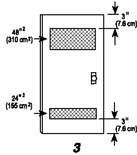
1. Recessed Area 2. Side view - closet or confined area 3. Closet door with vents
