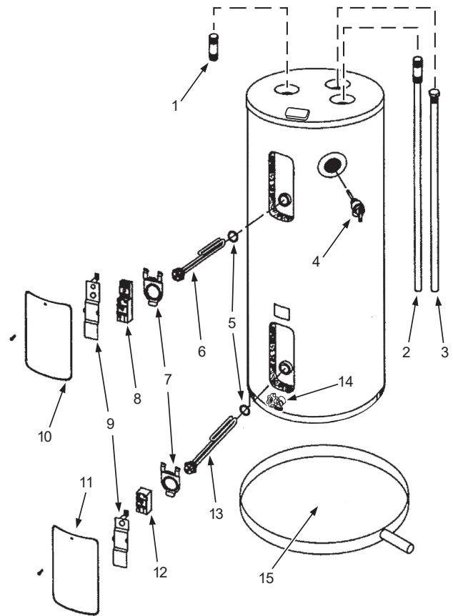
Figure 7. Repair Parts
