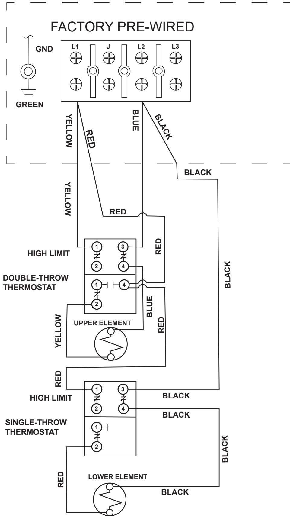
Figure 9. Wiring Diagram
