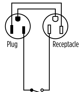
Vertical Switch with Piggyback Plug
