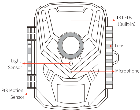
Figure 1: Front View
