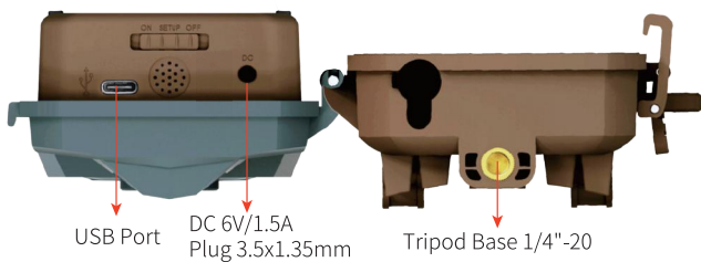
Figure 2: Bottom View
