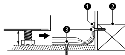
1 Anti-tip Bracket
