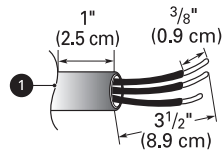
1 Cord/Conduit connection plate
