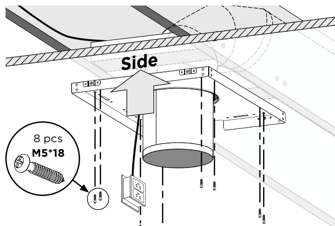
3.1 Side Vent - Floor above
