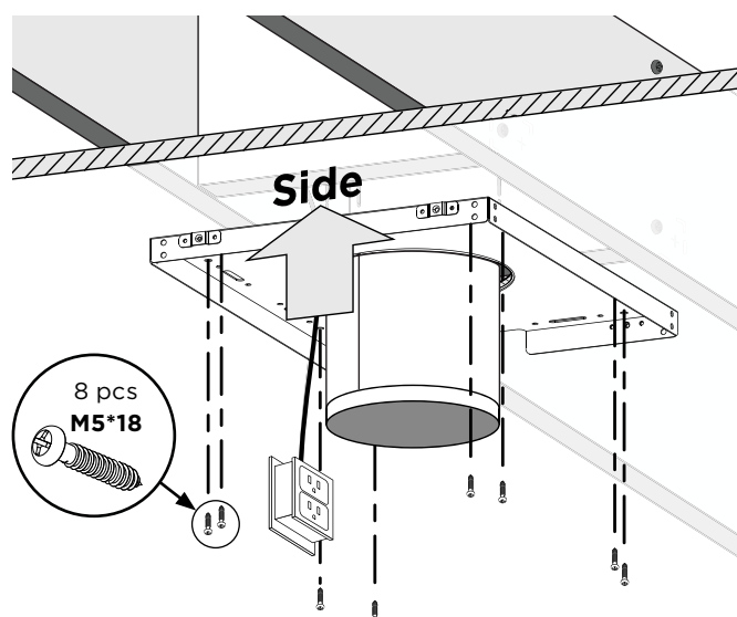
3.2 Roof Vent - No floor above
