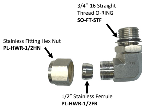
PL-MTE-3/4SX1/2SL 4"-16S X 1/2" TUBE 90DEG. SS316L
