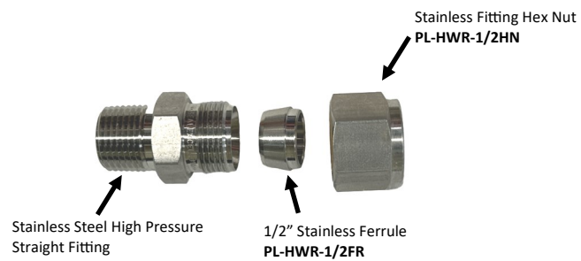
PL-MTS-3/8X1/2SL 3/8" NPT X 1/2" TUBE FITTING ST. SS316L
