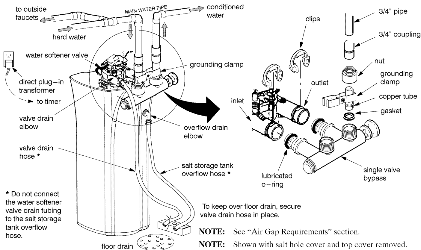
Figure 5 (typical installation)
