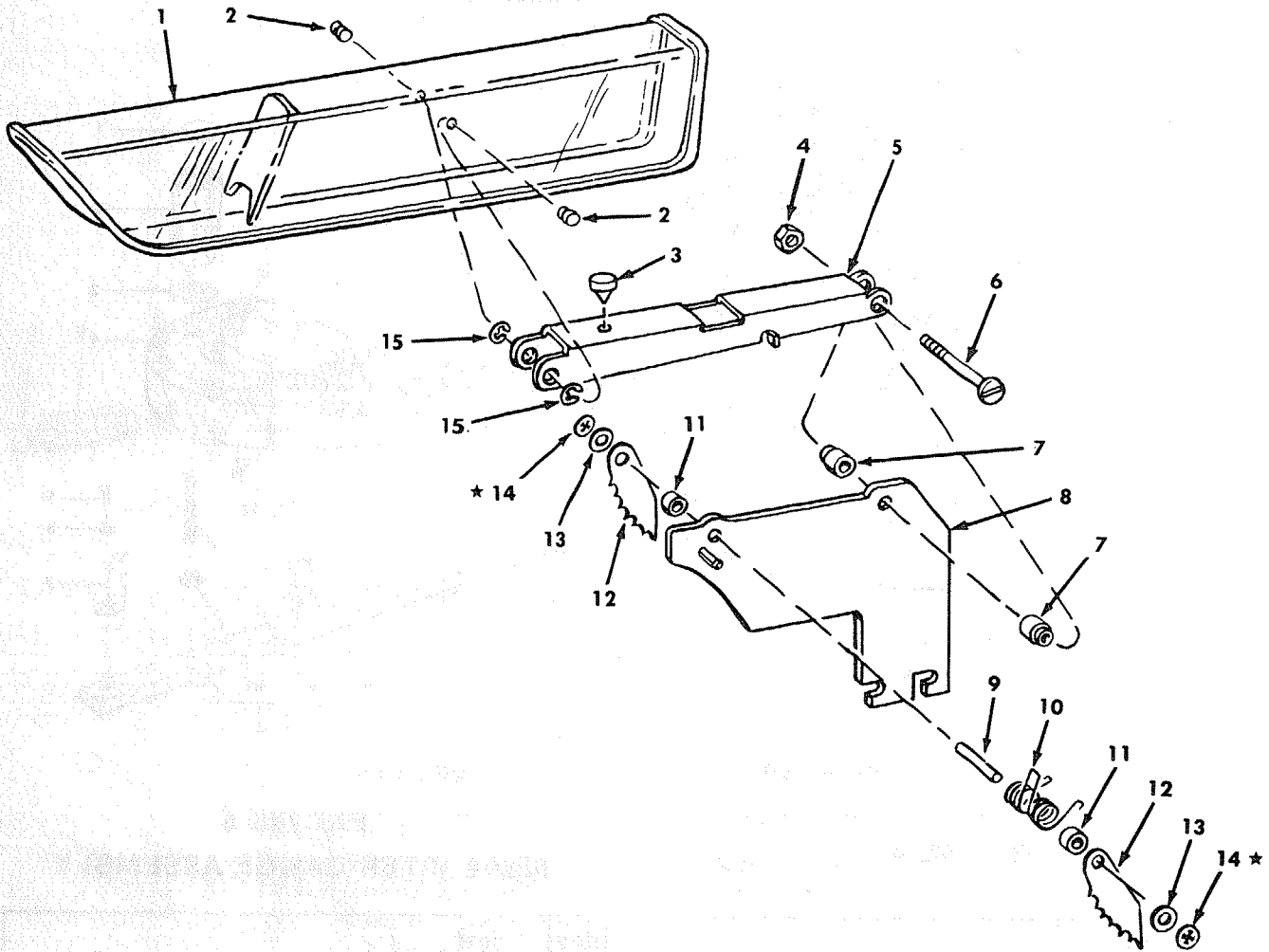
FIGURE 6 — 62805 GUARD ASSEMBLY
