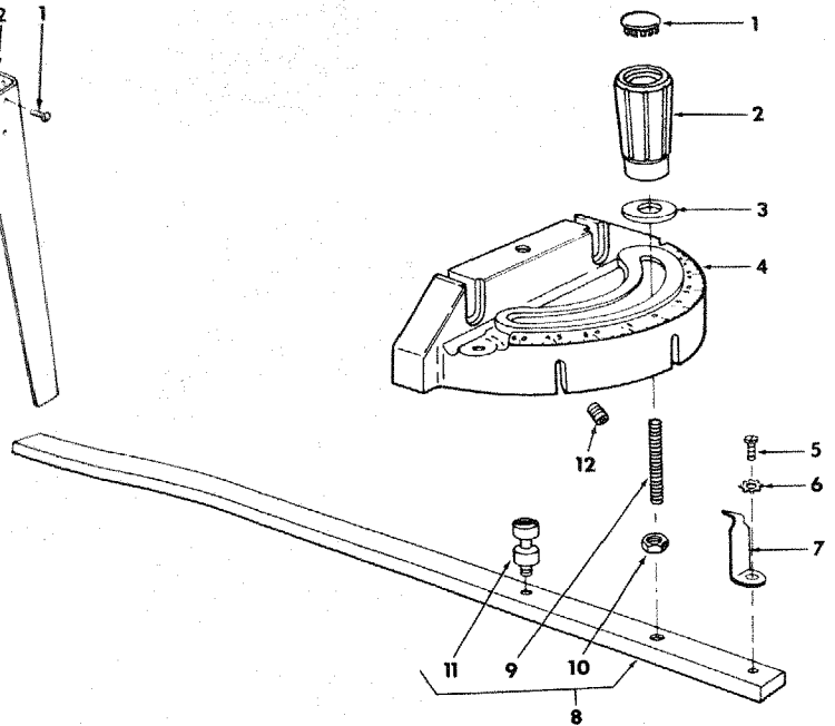
FIGURE 5 62694 MITER GAUGE ASSEMBLY
