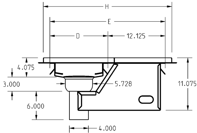
End View of Cool Trough®
