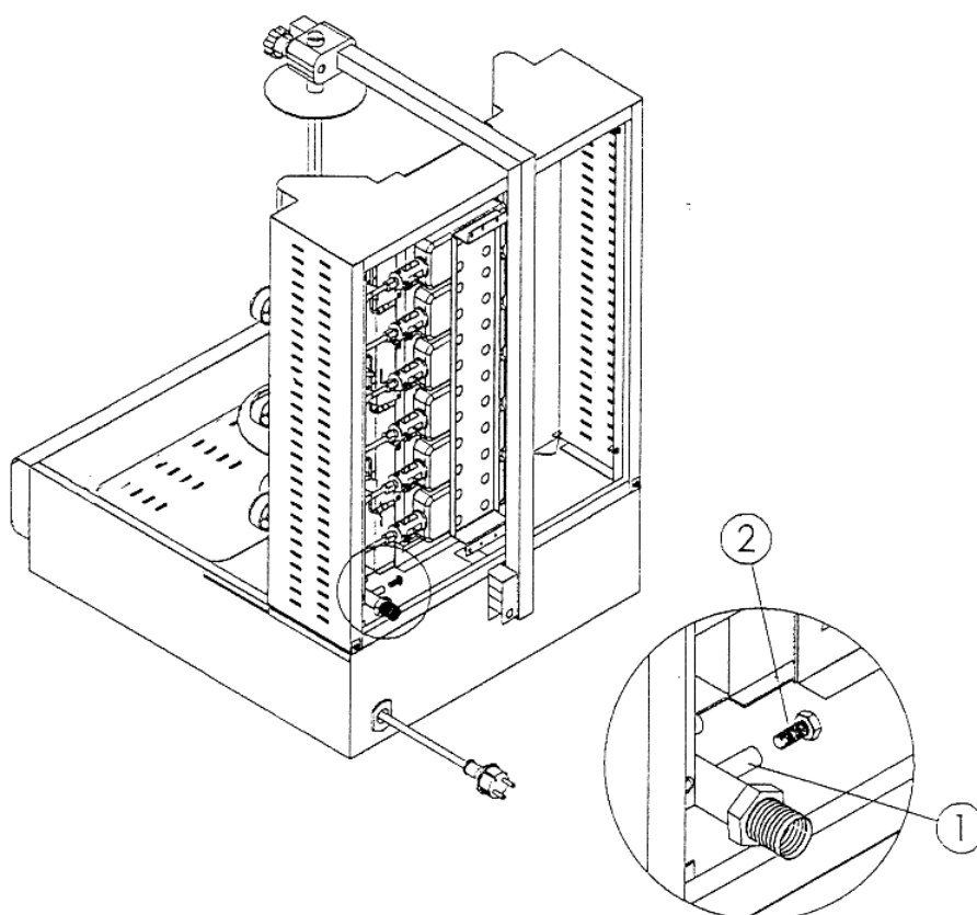
Fig. 1: Pressure control
