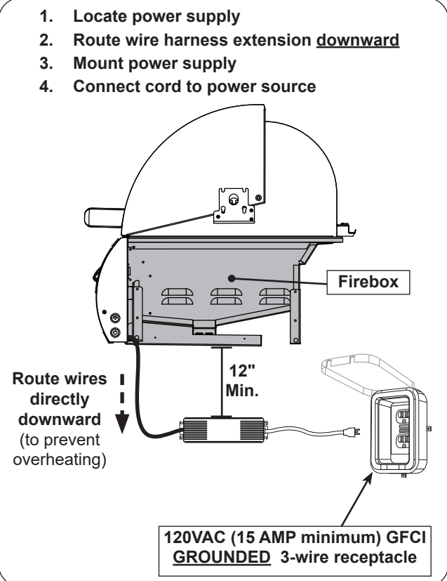
Fig. 30-3 Electrical installation
