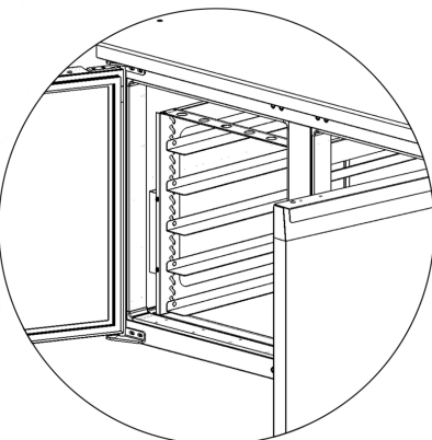
FIGURE 18C: Pan Slide Cage - Install Angle Slides
