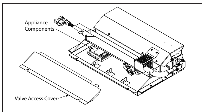
Figure 6.1 Burner Assembly
