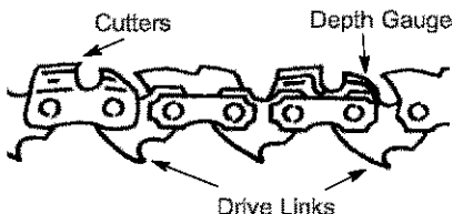
CUTTERS MUST FACE IN DIRECTION OF ROTATION
