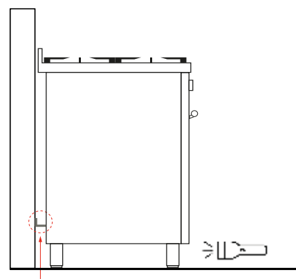
Anti-tip bracket
