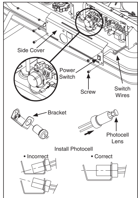
Figure 18. Photocell Replacement
