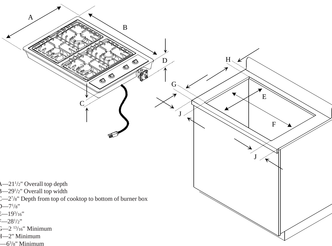
Cooktop and Countertop Dimensions
