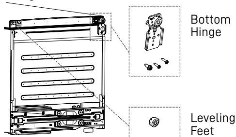
Refrigerator Bottom
