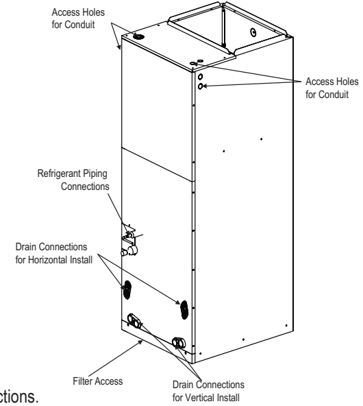
Figure 252: General and Duct Connection Dimensions.
