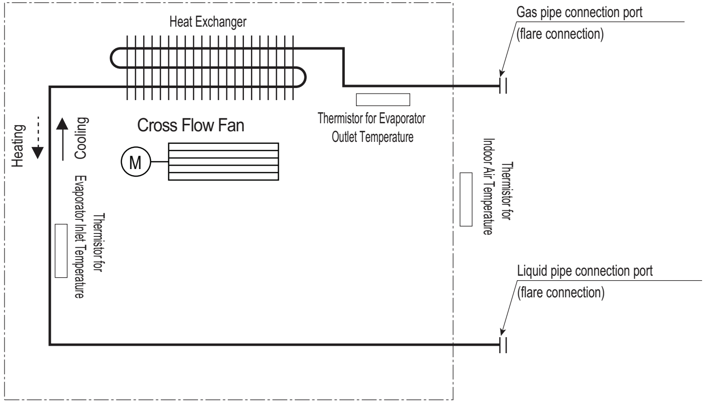
Figure 219: Multi F Vertical-Horizontal Air Handling Indoor Unit Refrigerant Flow Diagram.
