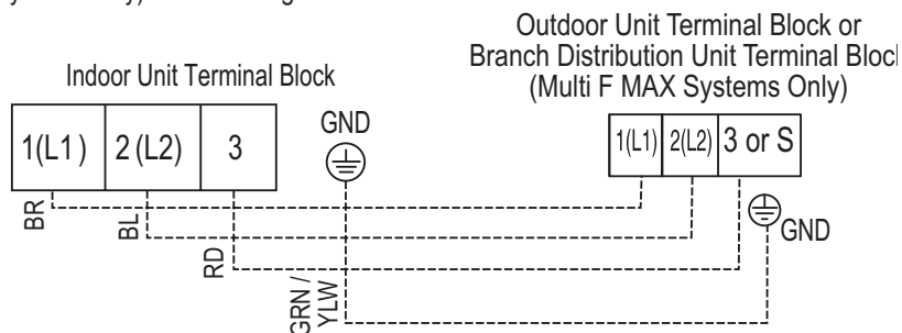
Figure 236: Indoor Unit to Outdoor Unit / Branch Distribution Unit (Multi F MAX systems only) Power Wiring / Communications Cable Connections.
