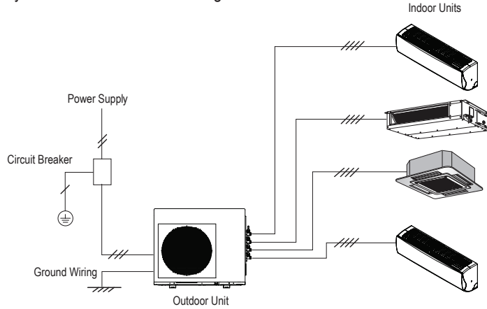
Figure 285: Typical Multi F System General Power / Communications System Schematic When Wiring is Less Than 130 Feet.
