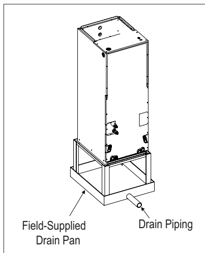
Figure 259: Typical Vertical Up/Down Installation Drain System.
