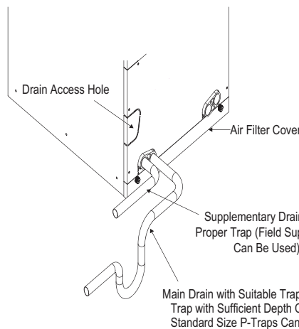
Figure 263: Vertical Primary and Secondary Drain Layout.
