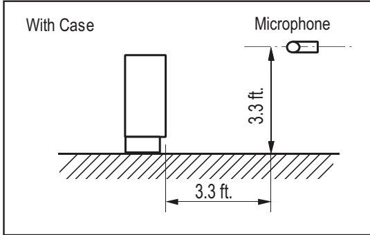
Figure 217: Sound Pressure Level Measurement Location.
