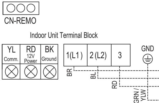
Figure 270:Wired Controller Connection on the Indoor Unit Terminal Block.
