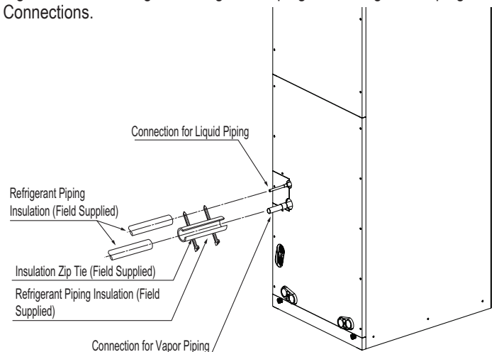
Figure 266: Insulating the Refrigerant Piping and Refrigerant Piping Connections.
