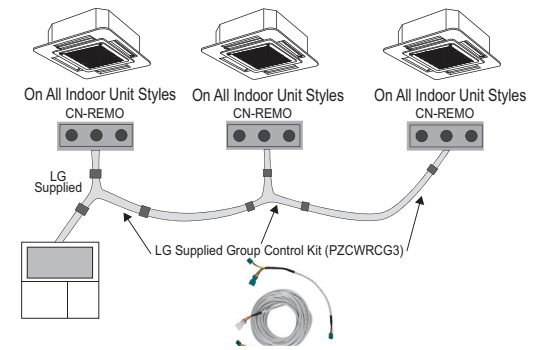
Figure 303: Example of Indoor Unit Group to Zone Controller Connections (CN-REMO).
