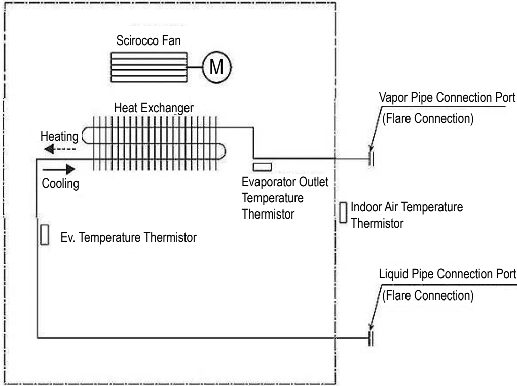
Figure 249: Four-way Vertical-Horizontal Air Handling Indoor Unit Refrigerant Flow Diagram.
