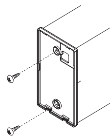
Figure 273: Attaching the Wall Plate.
