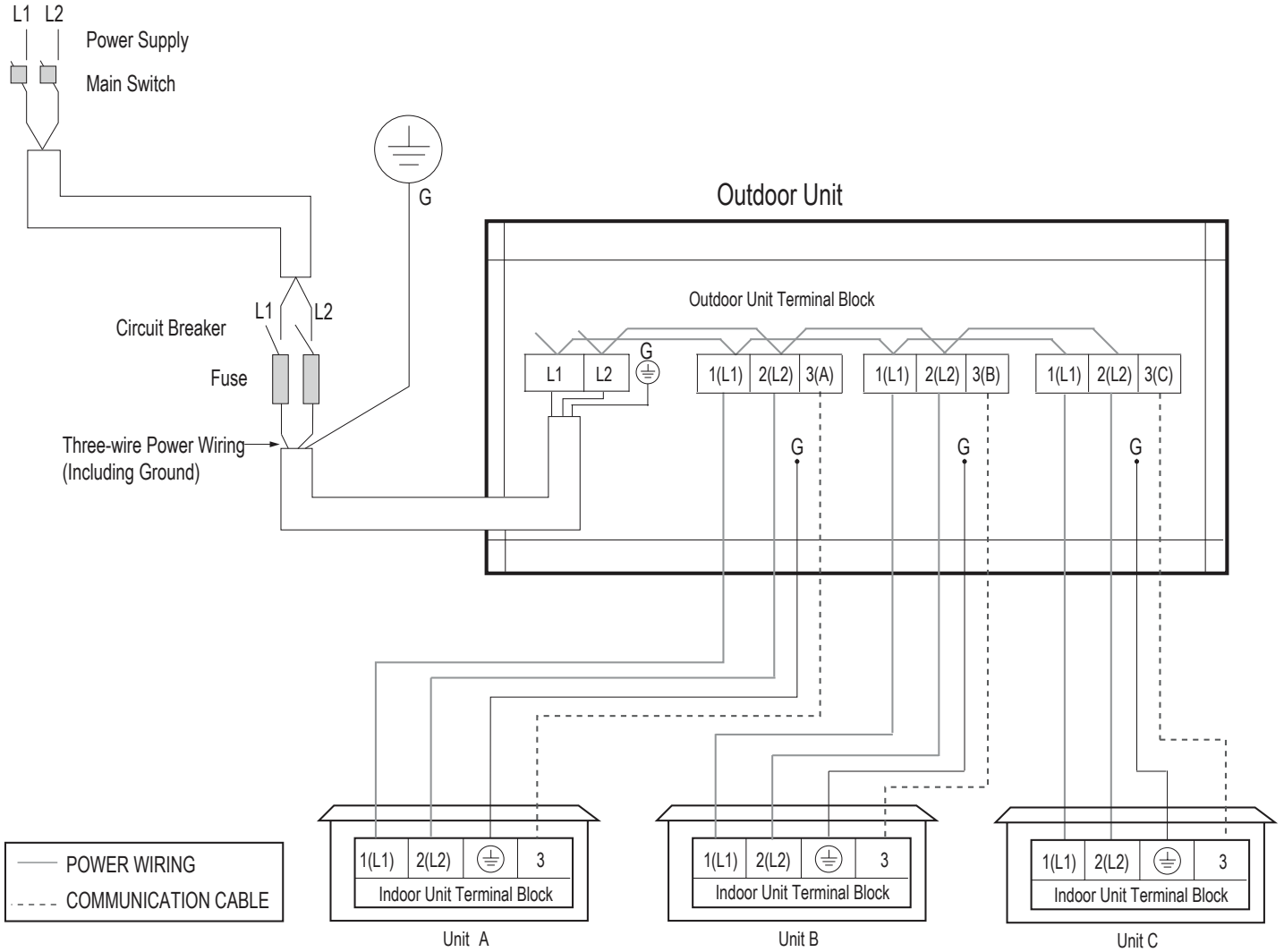
Figure 297: Multi F with LGRED LMU240HHV System Power Wiring and Communications Cable Connections.
