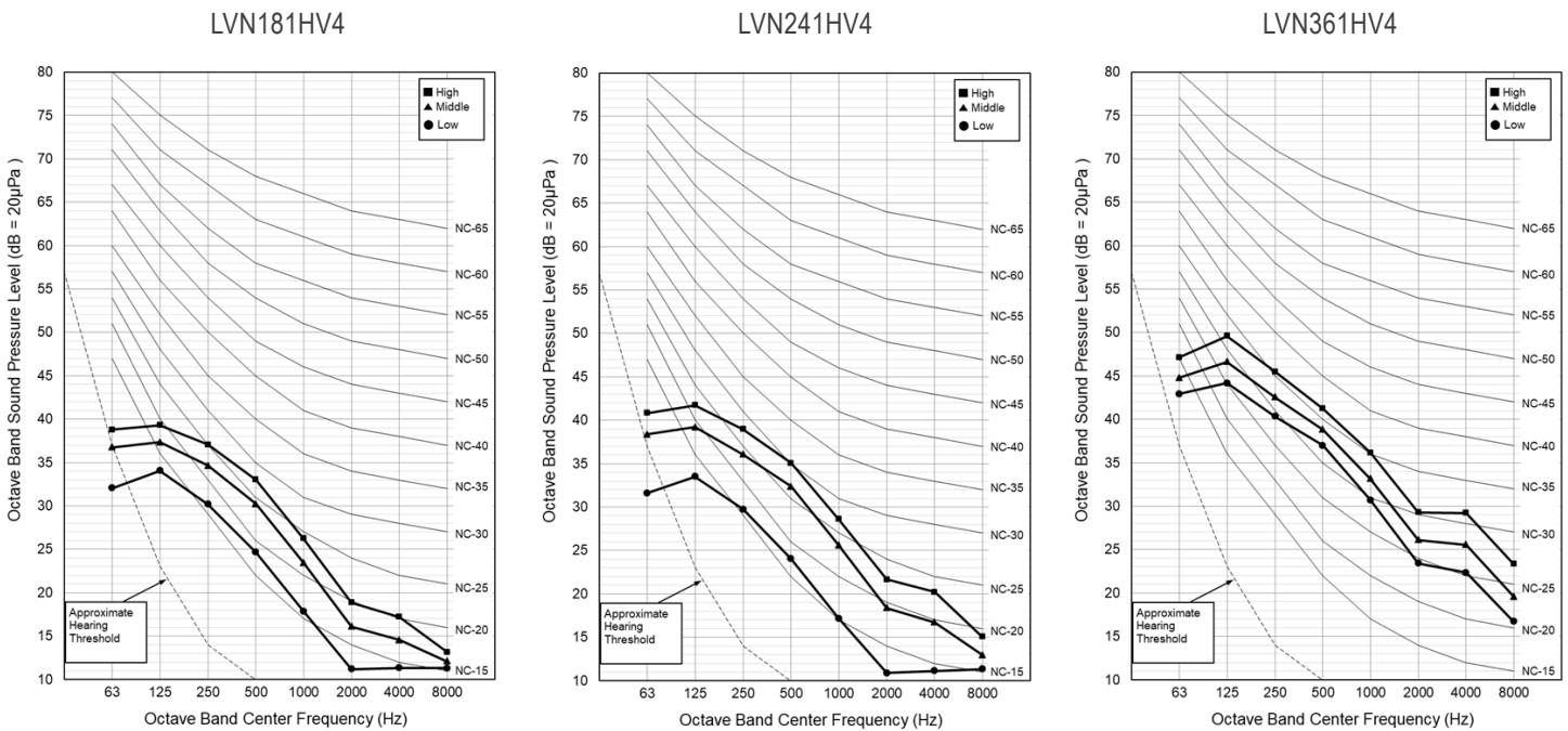
Figure 247: Sound Pressure Level Diagrams.
