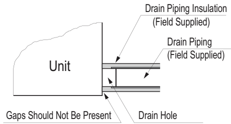
Figure 261: Close up of Drain Piping Connection.
