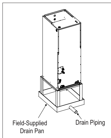
Figure 227: Vertical Installation Drain System.
