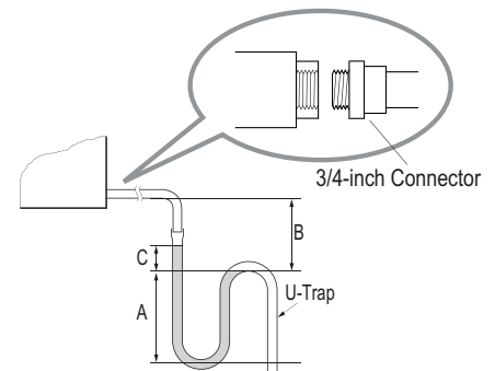
Figure 262: Installing the U-Trap.
