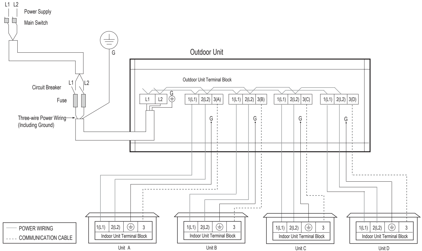
Figure 298: Multi F with LGRED LMU300HHV System Power Wiring and Communications Cable Connections.
