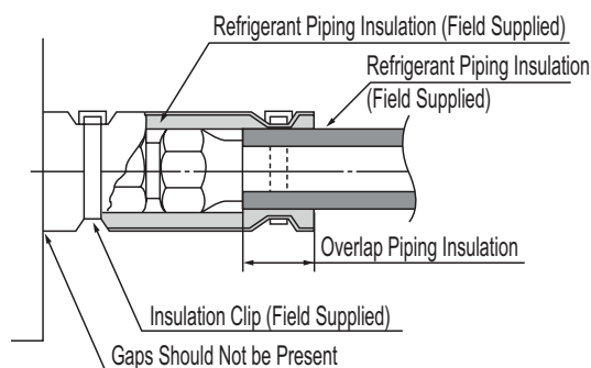
Figure 233: Close Up of Refrigerant Piping Connection Insulation.
