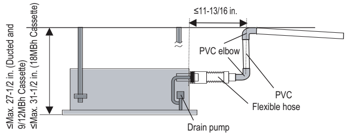
Figure 281: Diagram of an Indoor Unit with a Drain Pump.
