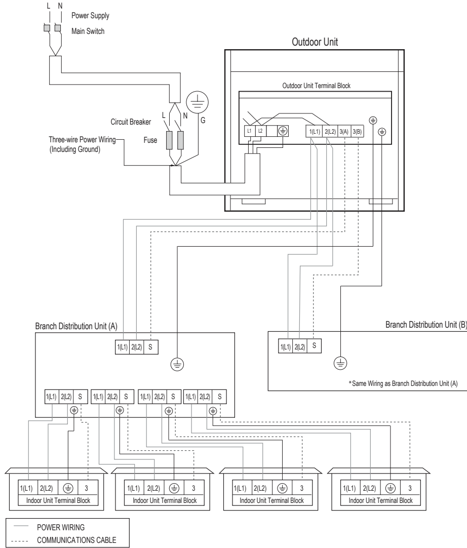
Figure 299: Multi F MAX with LGRED LMU360HHV and LMU420HHV System Power Wiring and Communications Cable Connections.
