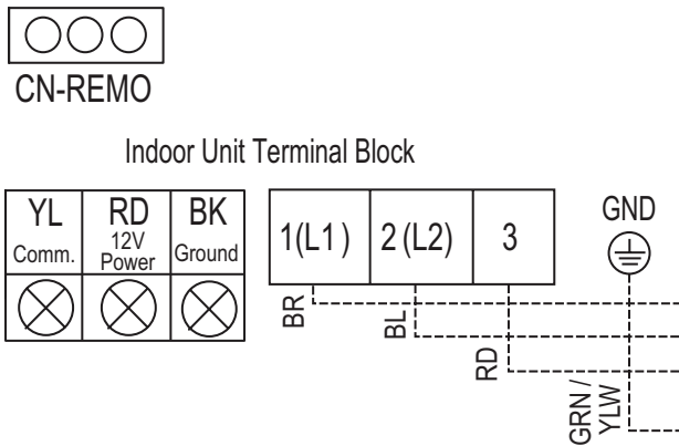
Figure 238: Wired Controller Connection on the Indoor Unit Terminal Block.
