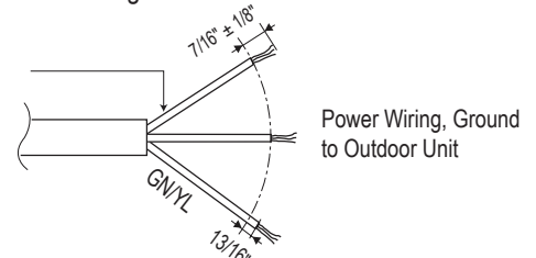
Figure 282: Multi F / Multi F MAX Outdoor Unit Power Wiring.
