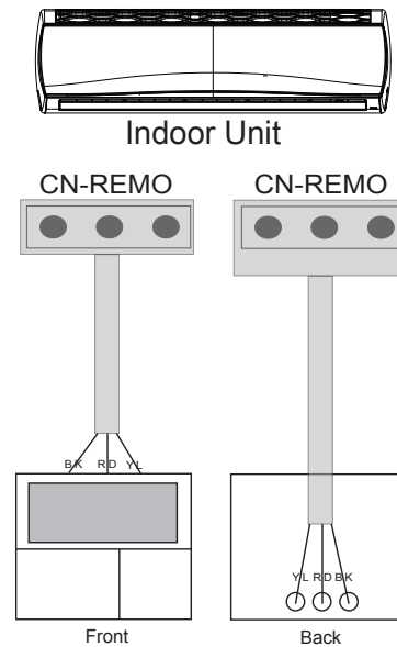
Figure 301: Another Example of Indoor Unit to Zone Controller Connection.
