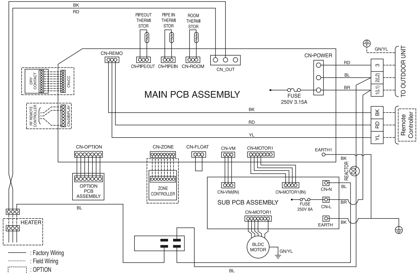
Figure 220: Multi F Vertical-Horizontal Air-Handling Indoor Unit Wiring Diagram.
