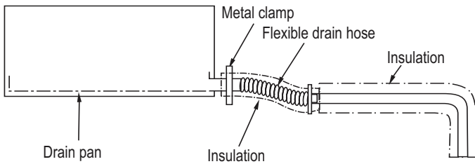
Figure 280: Diagram of an Indoor Unit with a Gravity Drain.
