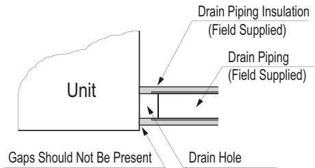
Figure 229: Close up of Drain Piping Connection.
