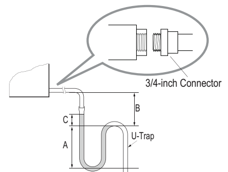
Figure 230: Installing the U-Trap.
