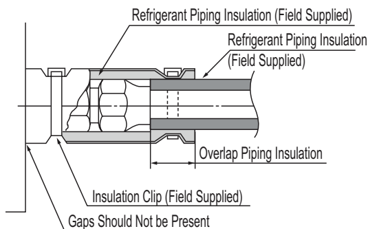
Figure 265: Close Up of Refrigerant Piping Connection Insulation.
