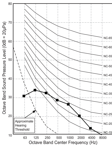
Figure 123: Sound Pressure Level Diagrams. LDN097HV4
