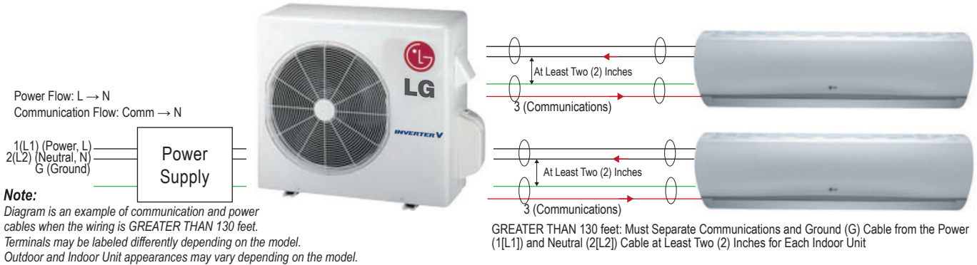
Figure 288: Schematic of a Multi F MAX with LGRED System When the Wiring is GREATER THAN 130 Feet.
