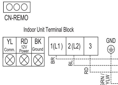
Figure 173: Wired Controller Connections on the Indoor Unit Terminal Block.
