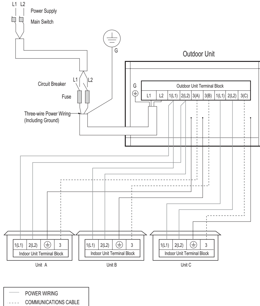
Figure 290: Multi F LMU24CHV System Power Wiring and Communications Cable.
