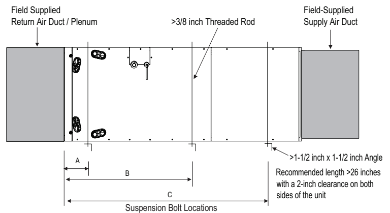
Figure 257: Typical Horizontal Right Installation.
