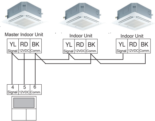
Figure 302: Example of Indoor Unit Group to Zone Controller Connections (Sig-12V-GND [Comm.] Terminal).
