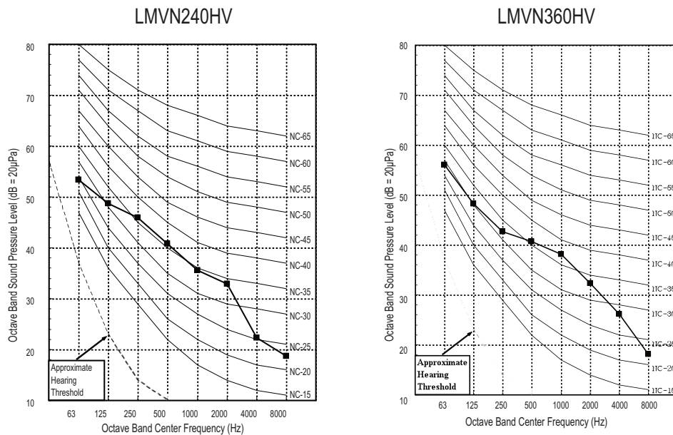
Figure 218: Sound Pressure Level Diagrams.
