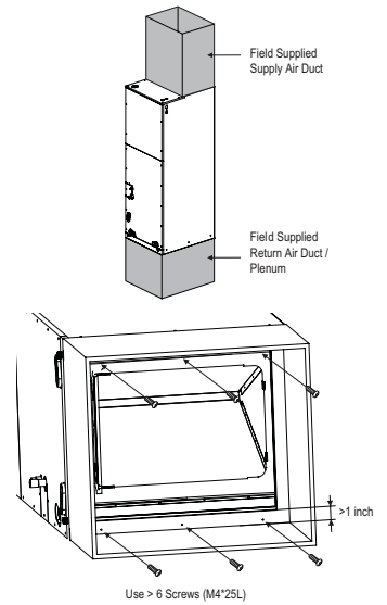
Figure 254: Vertical Installation / Attaching the Bottom Duct.
