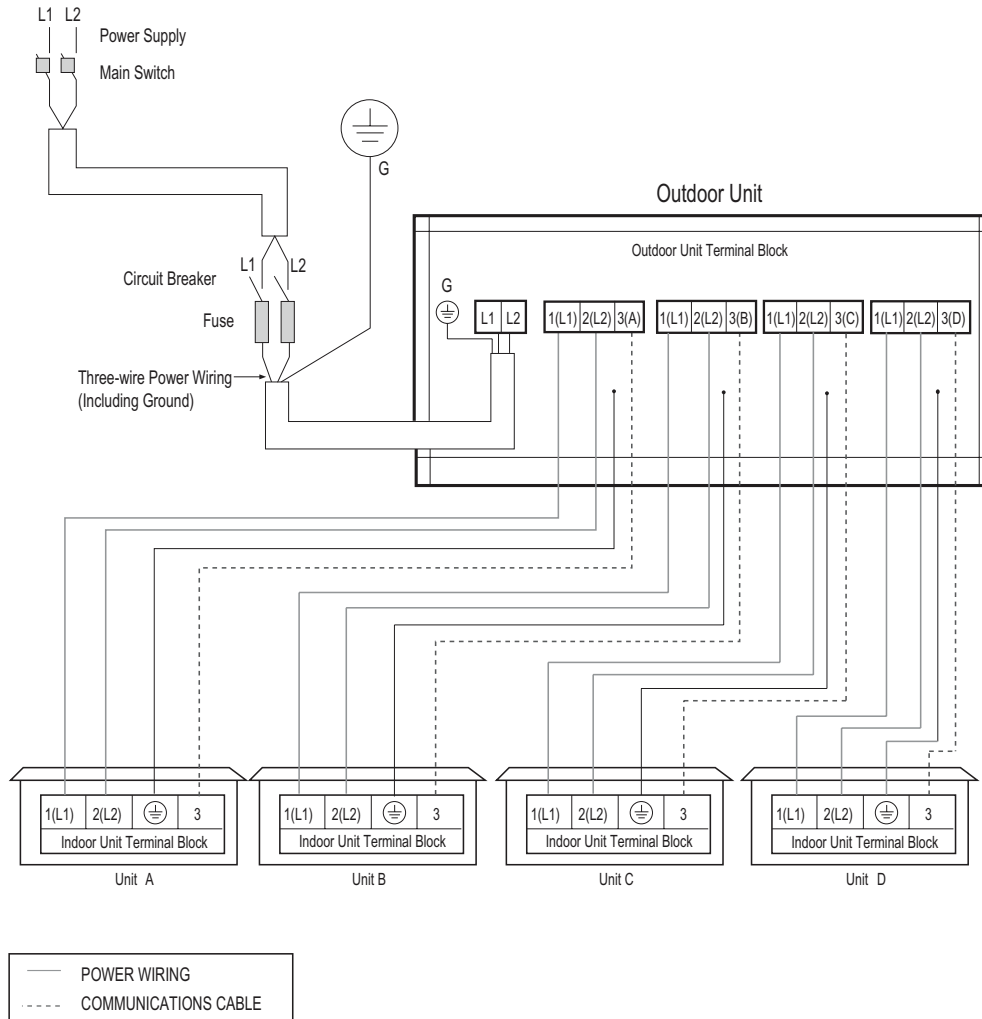
Figure 291: Multi F LMU30CHV and LMU36CHV System Power Wiring and Communications Cable.
