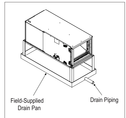
Figure 260: Typical Horizontal Left/Right Installation Drain System.
