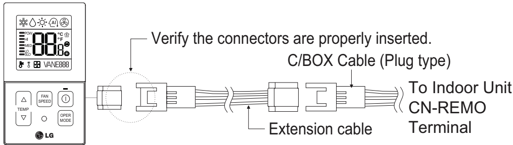
Figure 237: PZCWRC1 LG Wired Remote Extension Cable.
