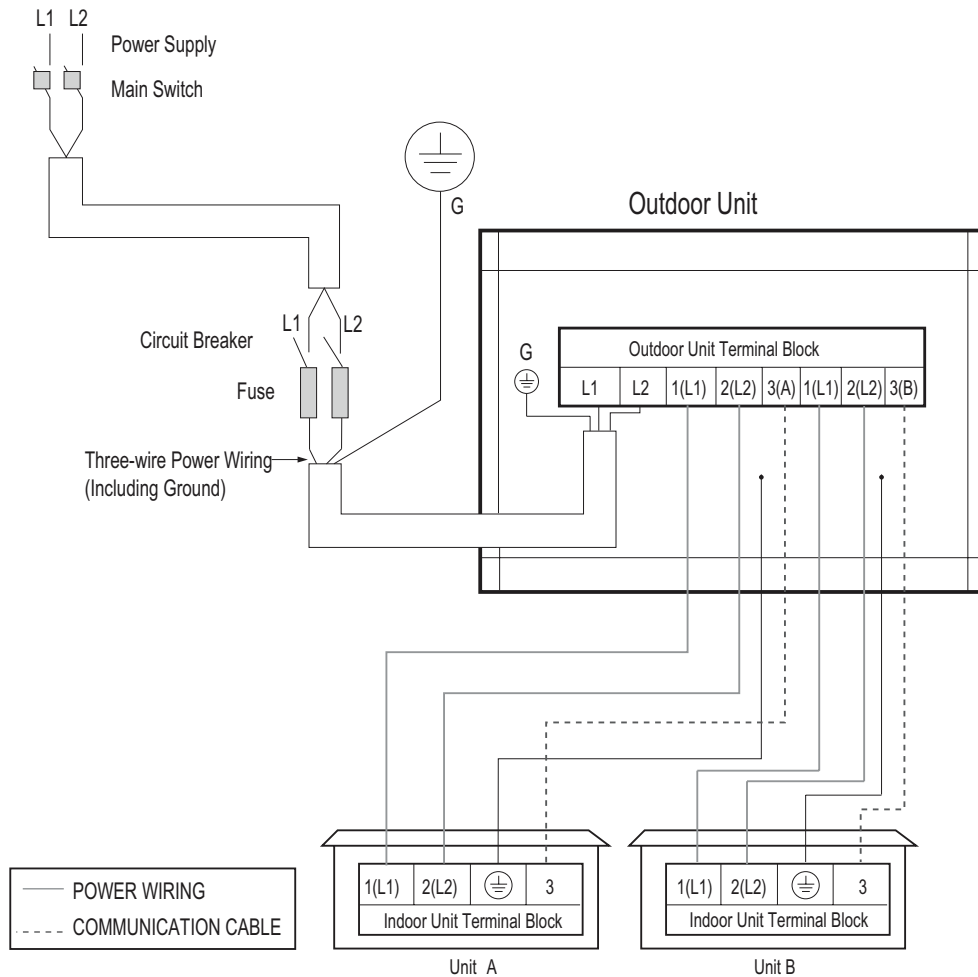
Figure 289: Multi F LMU18CHV System Power Wiring and Communications Cable.
