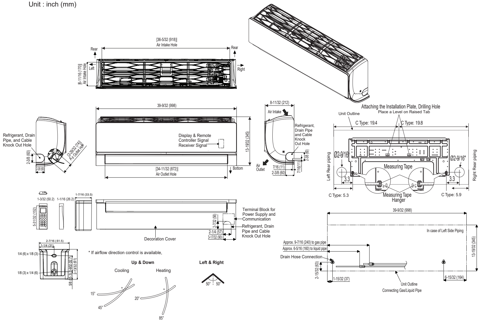
Figure 3: LAN180HSV5 Dimensions.
