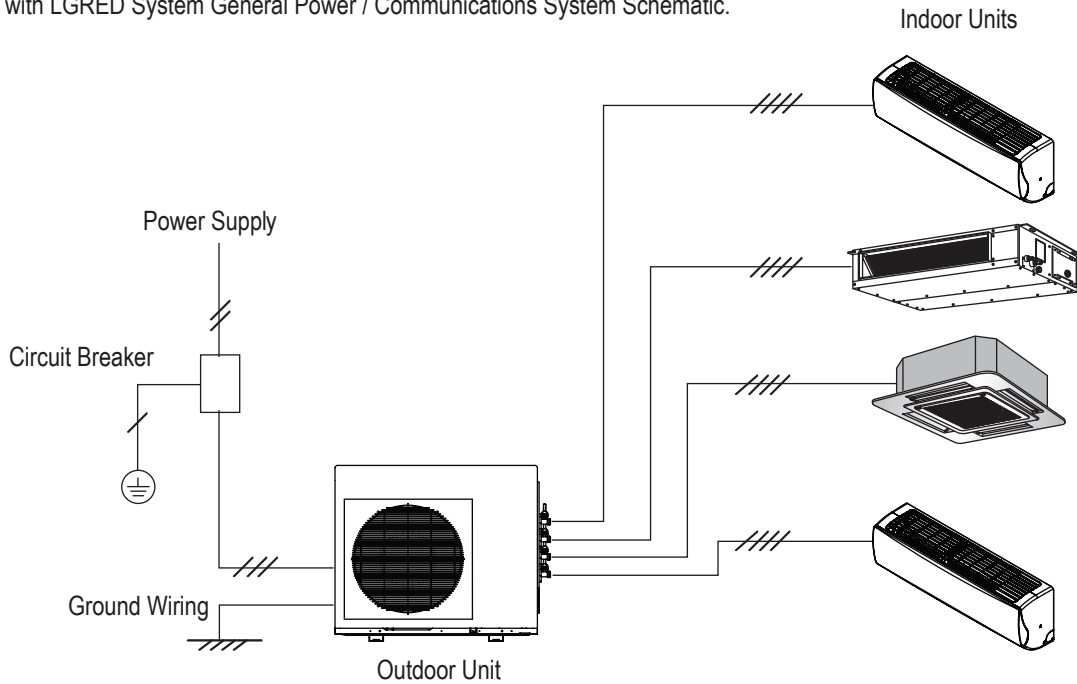
Figure 295: Multi F MAX with LGRED System General Power / Communications System Schematic.
