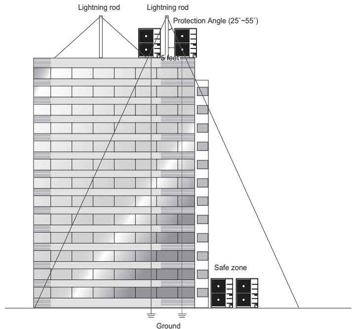
Figure 279: Lightning Protection Diagram.
