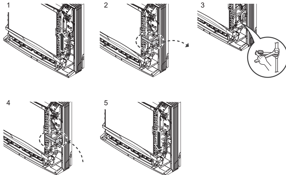
Figure 109: Pipe Connection.
