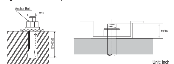
Figure 278: Close up of Bolt Attachment.
