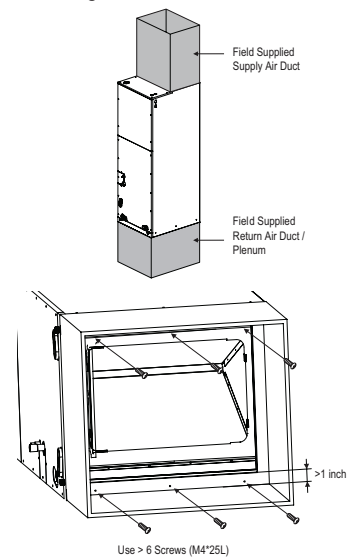
Figure 224: Vertical Installation / Attaching the Bottom Duct.
