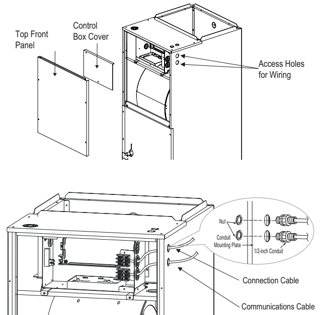
Figure 267: Connecting the Power Wiring and Communications Cable.
