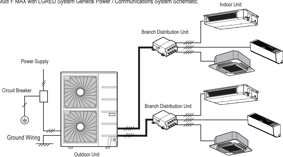
Figure 295: Multi F MAX with LGRED System General Power / Communications System Schematic.
