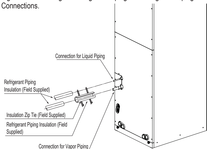
Figure 234: Insulating the Refrigerant Piping and Refrigerant Piping Connections.
