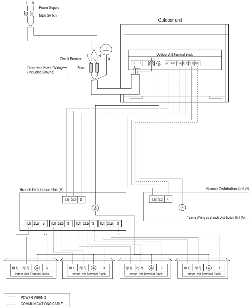
Figure 292: Multi F MAX LMU480HV and LMU540HV System Power Wiring and Communications Cable.
