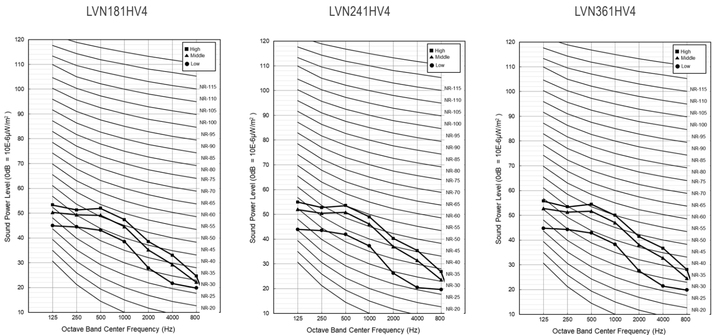
Figure 248: Sound Power Level Diagrams.
