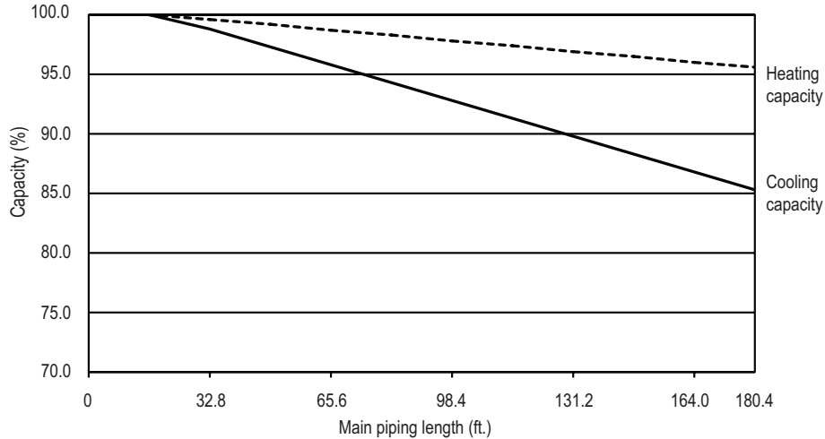
Figure 275: Multi F MAX / Multi F MAX with LGRED Outdoor Unit to Branch Distribution Unit Refrigerant Line Length Derate Chart.
