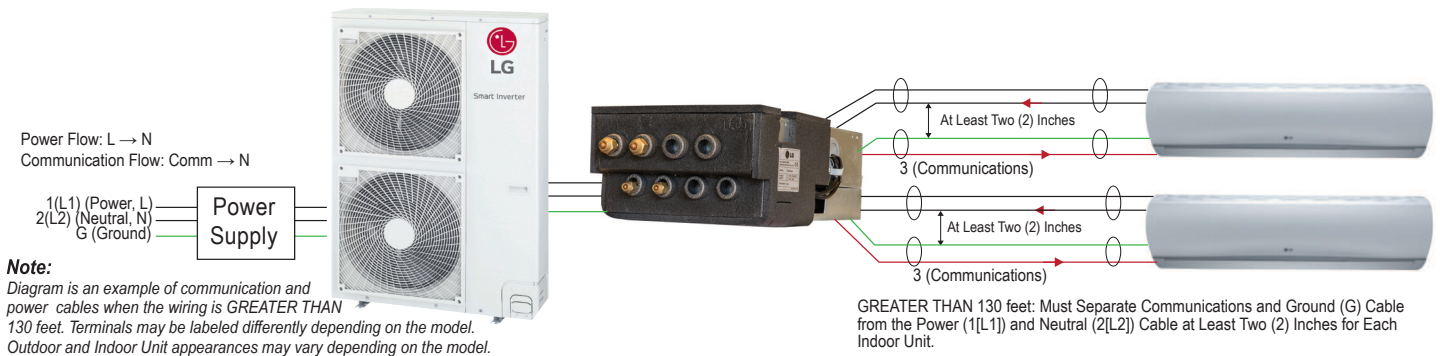
Figure 288: Schematic of a Multi F MAX with LGRED System When the Wiring is GREATER THAN 130 Feet.
