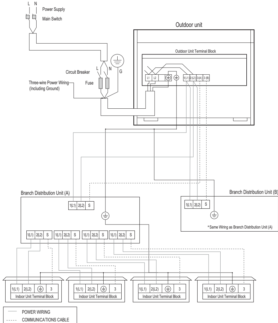
Figure 293: Multi F MAX LMU600HV System Power Wiring and Communications Cable.
