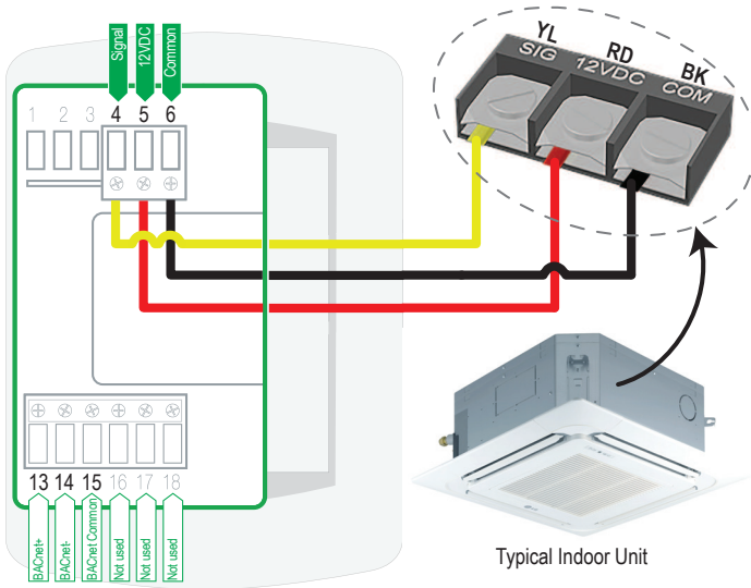
Figure 300: One Example of Indoor Unit to Zone Controller Connection.
