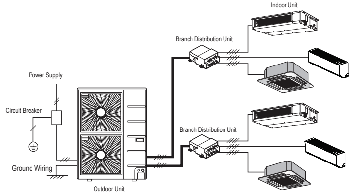
Figure 286: Typical Multi F MAX System General Power / Communications System Schematic When Wiring is Less Than 130 Feet.
