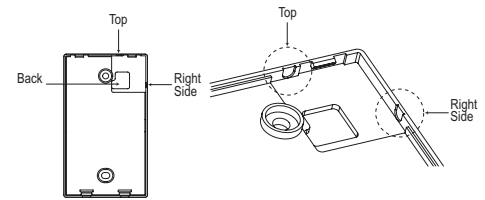
Figure 274: Installing / Removing the Controller.
