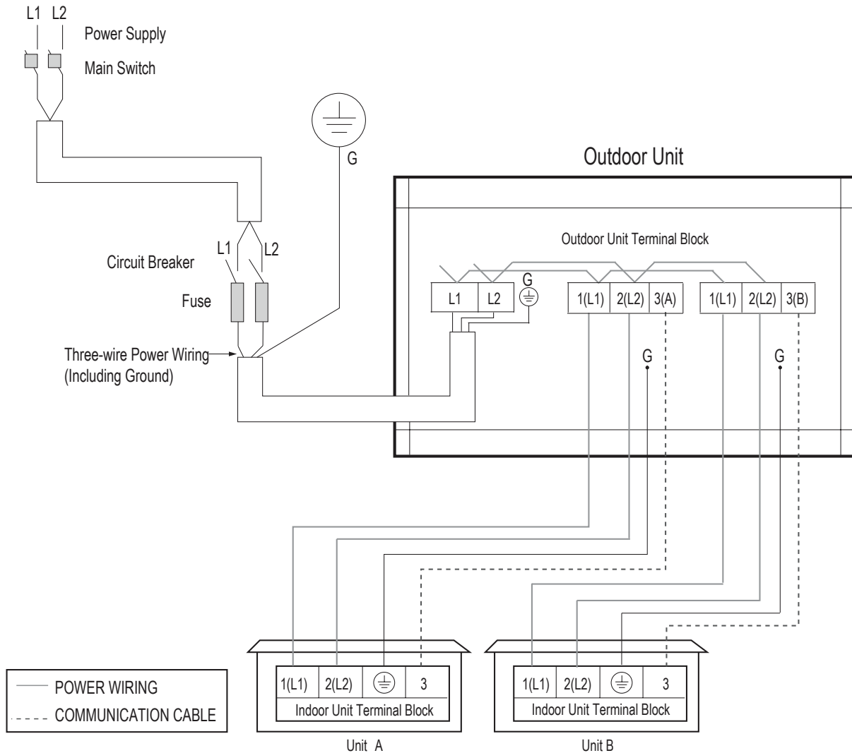
Figure 296: Multi F with LGRED LMU180HHV System Power Wiring and Communications Cable Connections.
