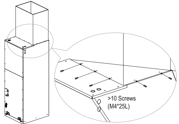
Figure 258: Securing the Ducts to the Unit.
