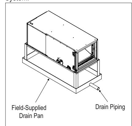
Figure 228: Horizontal Installation Drain System.
