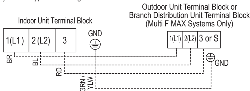
Figure 268: Indoor Unit to Outdoor Unit / Branch Distribution Unit (Multi F MAX systems only) Power Wiring / Communications Cable Connections.
