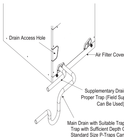
Figure 231: Vertical Primary and Secondary Drain Layout.
