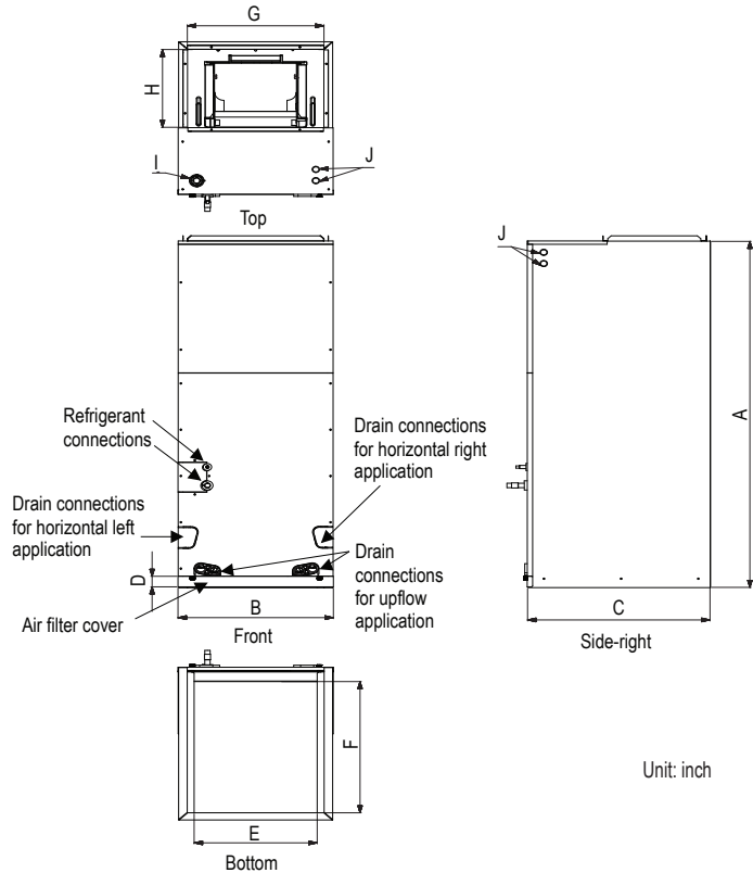
Figure 253: Location of Access Holes and Piping Connections.
