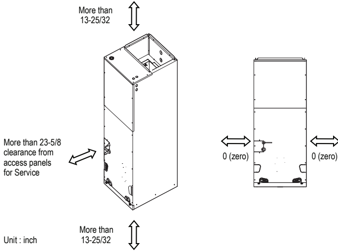
Figure 251: Clearance Requirements.
