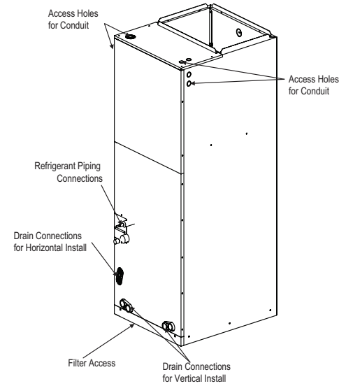
Figure 222: General and Duct Connection Dimensions.
