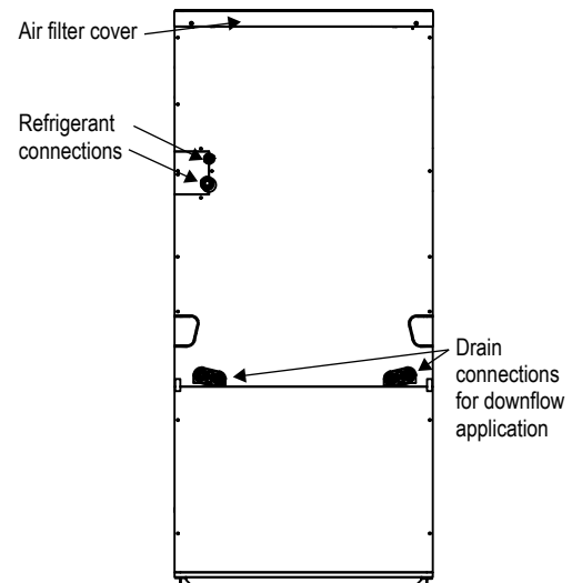
Figure 255: Chassis after Downflow Field Conversion.
