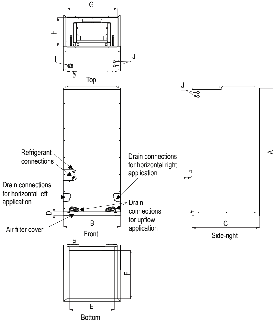
Figure 244: Four-way Vertical Air Handling Unit Dimensions.
