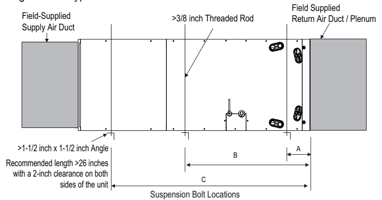
Figure 256: Typical Horizontal Left Installation.
