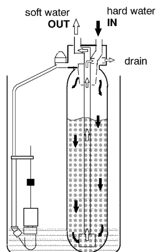
FIG. 9 Water Flow Through the Softener in Fast Rinse
