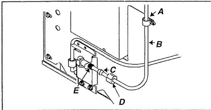
A "P" clamp B Copper tubing C Brass sleeve D Brass nut E Water valve inlet port
