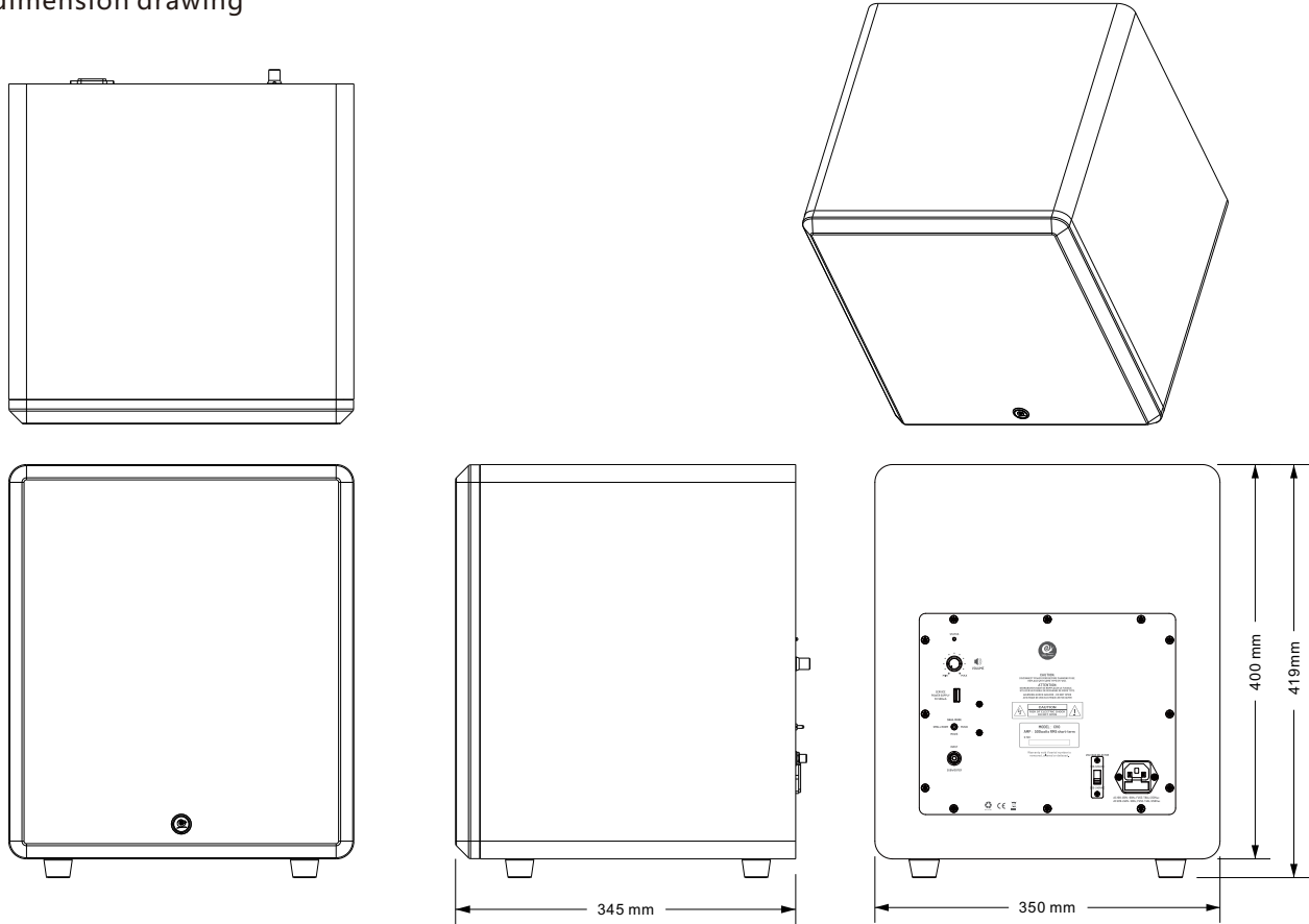
4: Finished dimension drawing
