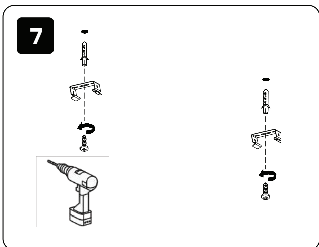
7. Fix the stainless steel bracket to the ceiling using screws and expansion anchors.
