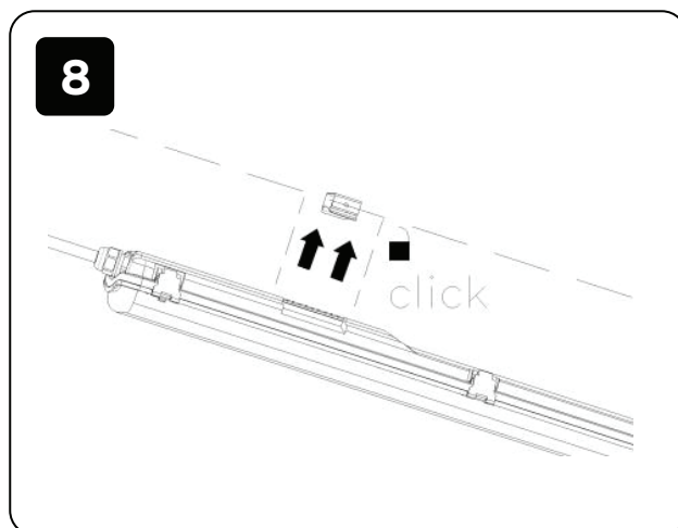
8. Mount the waterproof lamp onto the installed mounting brackets.
