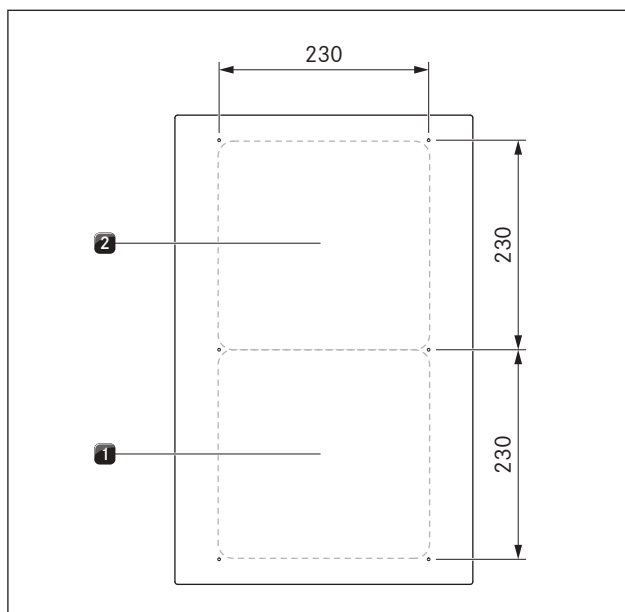
Fig. 4.7 Size of the cooking zones
