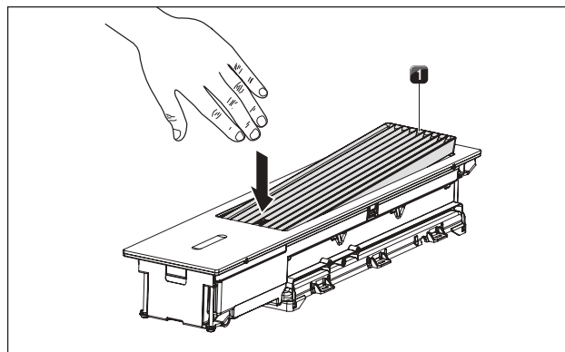
Fig. 9.1 Removing the air inlet nozzle
