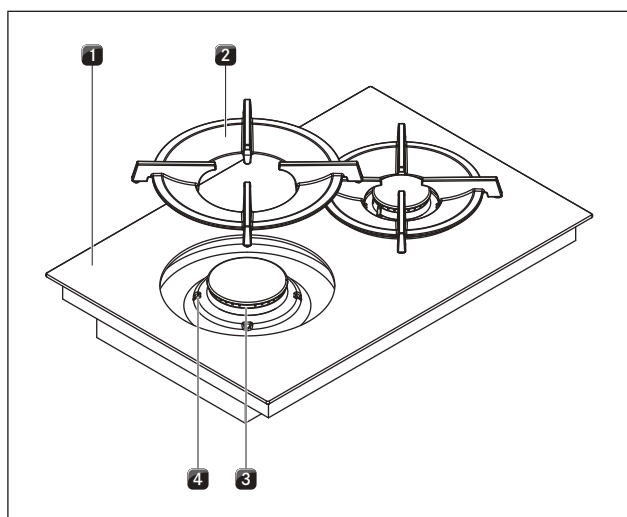
Fig. 9.1 Gas burner structure
