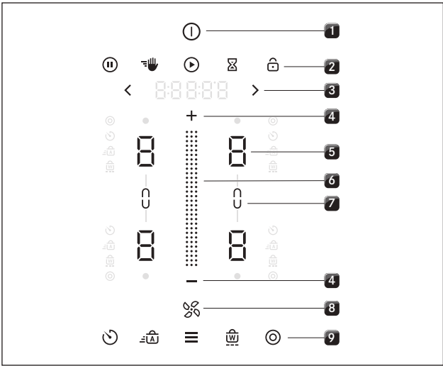
Fig. 4.2 Touch zones
