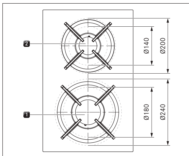
Fig. 4.17 Size of the cooking zones
