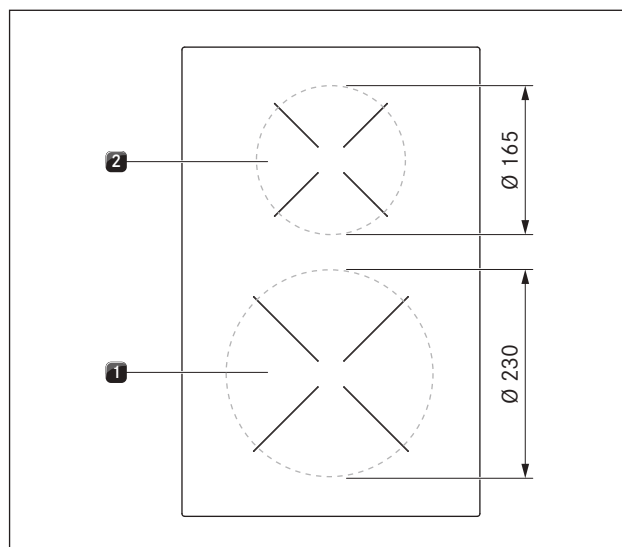
Fig. 4.9 Size of the cooking zones
