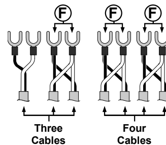
'Ezi connect' cable connector for water heater models: INFINITY 32, 26i, EVIROSMTART HD 250e, 200e (REU-VRM2632WC), 200i
