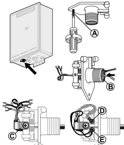
'Ezi connect' cable connector for water heater models: INFINITY 32, 26i, EVIROSMTART HD 250e, 200e (REU-VRM2632WC), 200i
