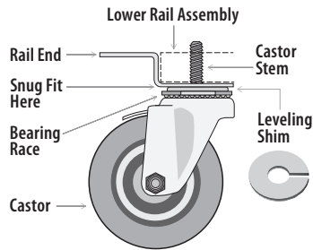
Fig. 7. Install shim(s).
