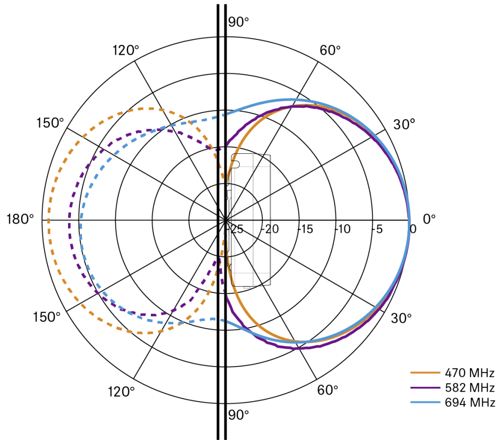
UHF (470 – 694 MHz) vertical [dB]
