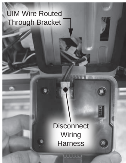
Figure 14 - Disconnecting UIM
