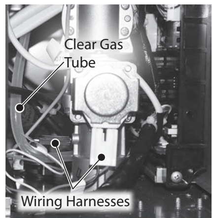
Figure 90 - Gas tube and wire harnesses
