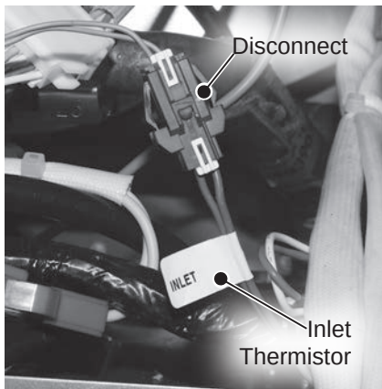
Figure 39 - Disconnecting inlet thermistor
