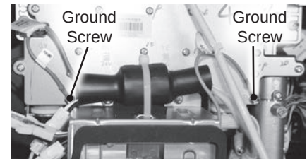
Figure 120 - Removing green ground wires
