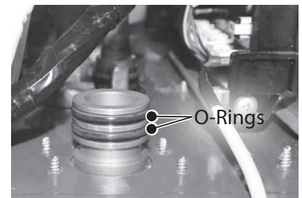
Figure 80 - Gas inlet connector O-rings
