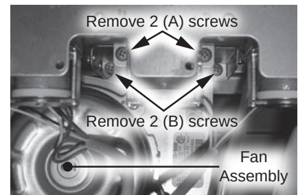
Figure 102 - Fan screw location (A & B)
