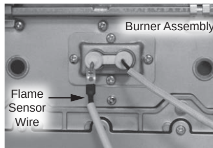
Figure 108 - Removing flame sensor wire
