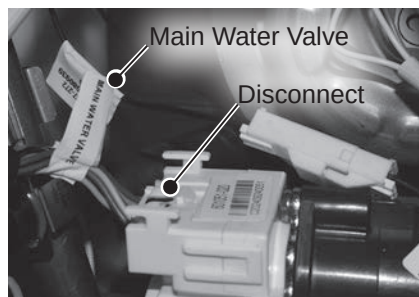
Figure 42 - Disconnecting main water valve
