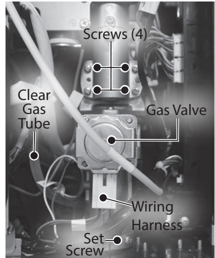
Figure 89 - Gas valve location and connections
