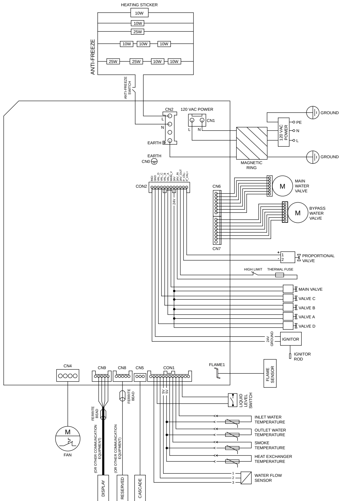
Figure 218 - Electrical wiring diagram
