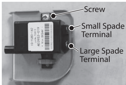
Figure 123 - Disconnecting ignitor assembly
