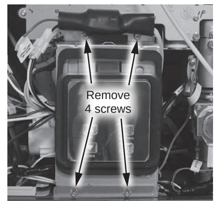
Figure 135 - Removing UIM and bracket screws
