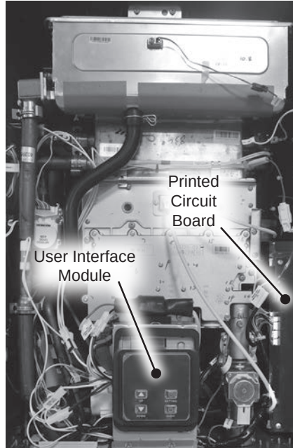
Figure 13 - Locating UIM
