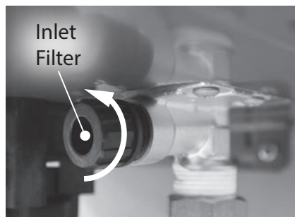
Figure 23 - Removing the inlet filter
