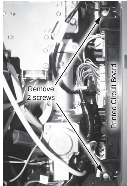
Figure 45 - Removing PCB screws
