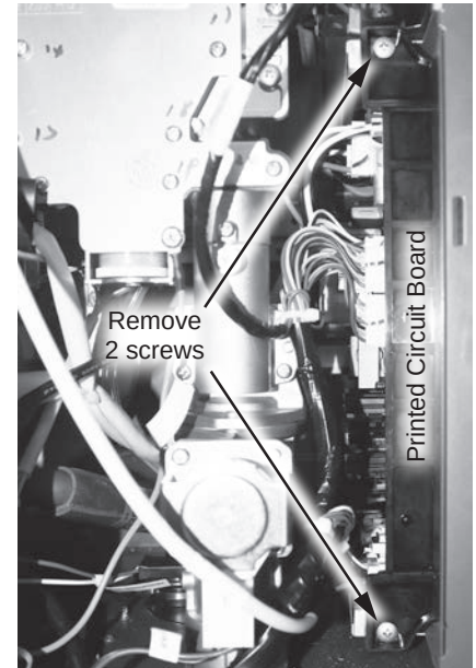
Figure 53 - Removing PCB screws
