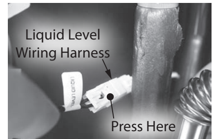
Figure 197 - Liquid level wiring harness location
