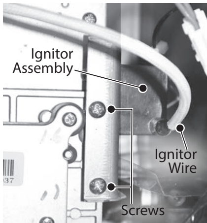
Figure 122 - Ignitor assembly location
