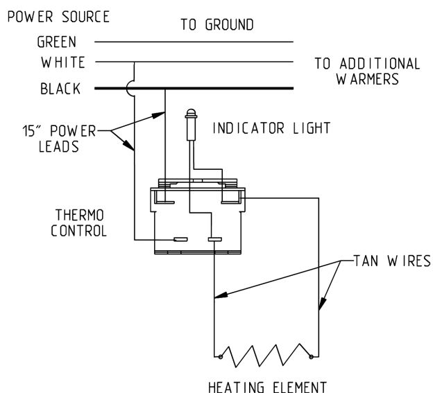
Wiring diagram - Thermostatic control
